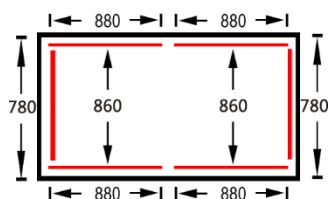
Diagrams of sealing beams position
